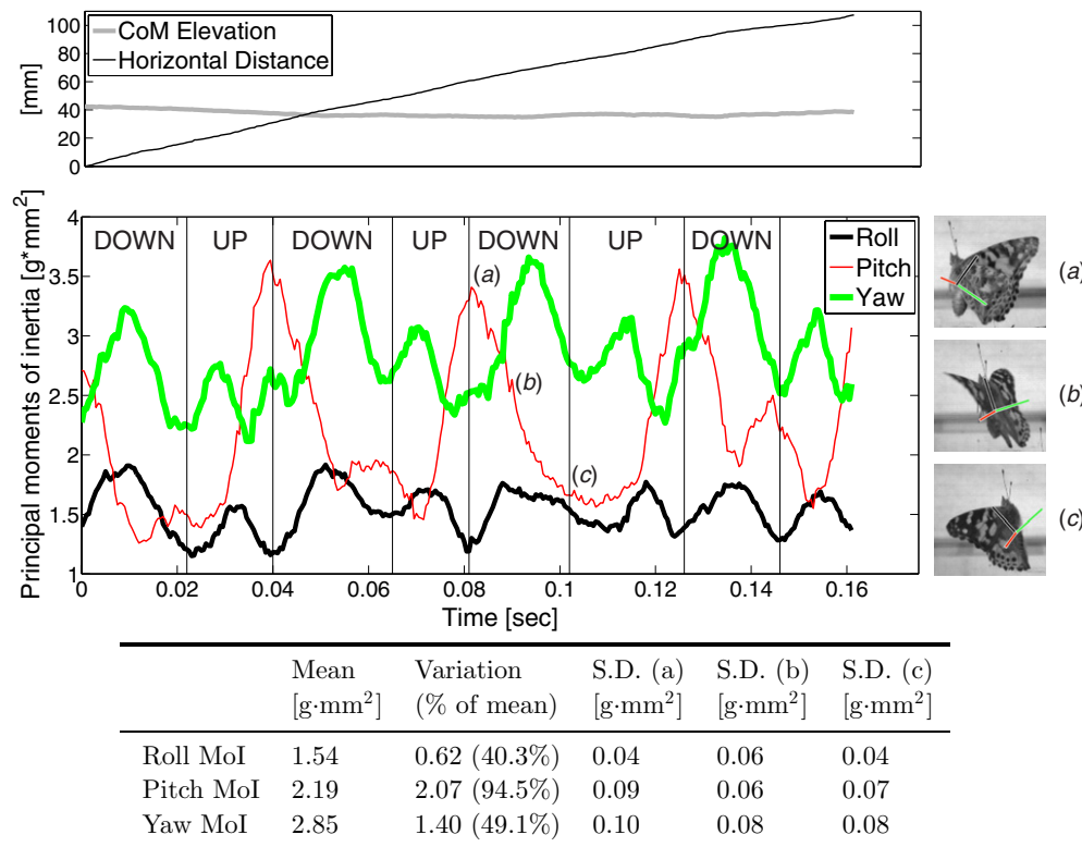
Figure 3. Temporal variation of the principal moments of inertia (MoIs) for a Painted Lady butterfly in forward flight over four wing flaps. Also shown are the time-mean values over the four wing flaps and the average variations that occur over each wing flap for each of the principal MoIs. The standard deviations are calculated for each of the principal MoIs at times (a), (b) and (c); time (a) corresponds to 0.0815 s, time (b) corresponds to 0.0935 s and time (c) corresponds to 0.101 s. In addition, the elevation of the insect CoM and the horizontal distance travelled by the CoM are plotted above.
