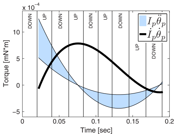
Figure 6. Components of rate of change of pitch angular momentum estimated using the upper and lower bounds of pitch MoI and the maximum time rate of change of MoI. Note that since the sign of I_p changes within each flapping cycle, the effect of I_p \dot{\theta}_p may be positive or negative throughout the manoeuvre.
