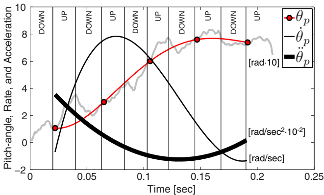
Figure 5. Pitch-angle \theta_p , rate \dot{\theta}_p and acceleration \ddot{\theta}_p estimated for a butterfly undergoing a manoeuvre that transitions from forward to climbing flight. Note that the pitch-angle is scaled by a factor of 10 and the pitch-acceleration is scaled by a factor of 10^{-2} .
